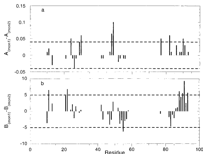
Figure 8. Comparison of the differences in (a) the NMR order parameters, expressed as A(\text{monomer 1}) - A(\text{monomer 2}) , where A = 1 - S^2 with (b) the differences in the X-ray B -factors for the backbone atoms, B(\text{monomer 1}) - B(\text{monomer 2}) , plotted as a function of residue number. The dashed lines in (a) are drawn at a level of \pm p_{sd} , where p_{sd} is the pairwise rmsd calculated using the estimated error of 0.02 in S^2 . In (b) the dashed lines are drawn at a level of \pm 5 \text{ \AA}^2 .
