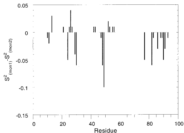
Figure 7. Plot summarizing the differences in order parameters of amides in the two HIV protease monomers, S^2(\text{monomer 1}) - S^2(\text{monomer 2}) , as a function of the residue number.
